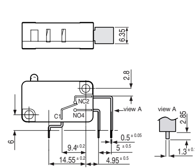
W3R2.5 for RAST 2.5 connector (SP9307)
